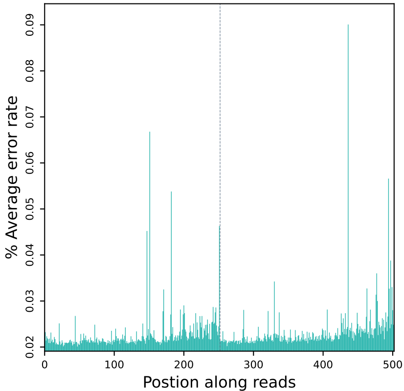
Error rate distribution along reads (R10626)
